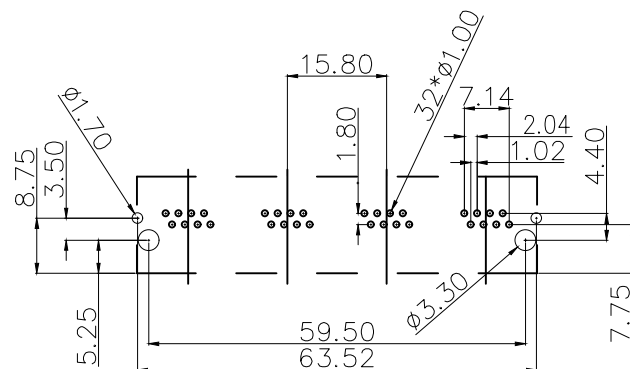
RECOMMENDED PCB LAYOUT TOP VIEW(TOL: ±0.05)
