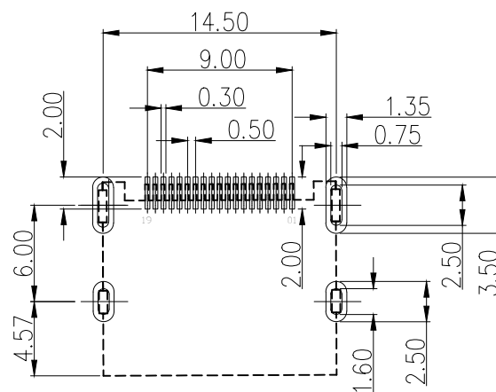
RECOMMEND PCB LAYOUT(±0.05)
