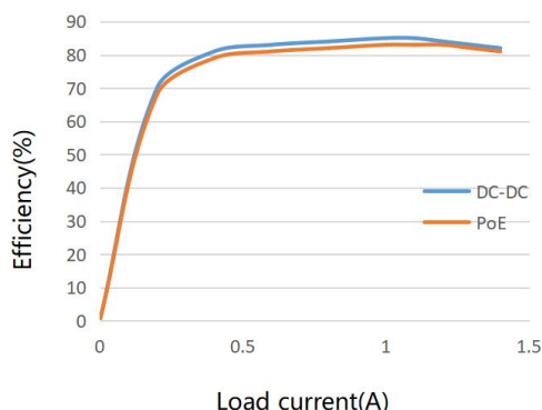
效率(Vout = 12V)
