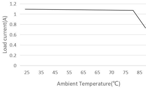
降额
