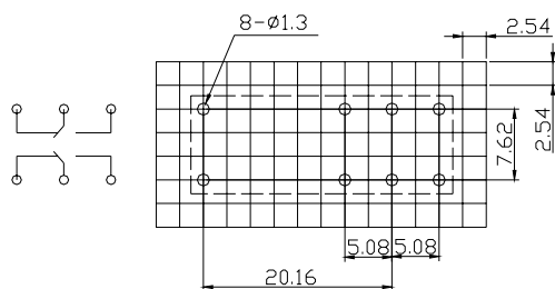
BOTTOM VIEW (2C)
