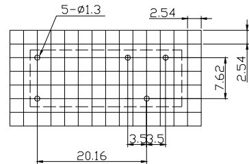
BOTTOM VIEW (1C)
