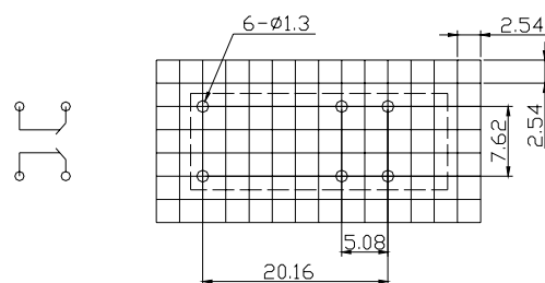
BOTTOM VIEW (2B)
