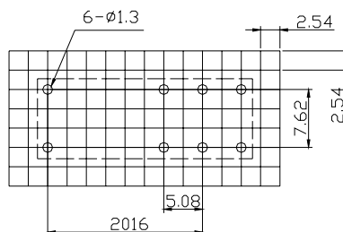
BOTTOM VIEW (1B)
