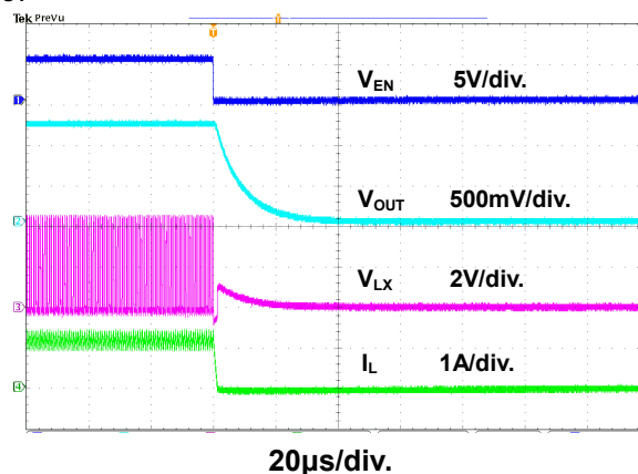
Figure 17. Power Off through EN Waveform
