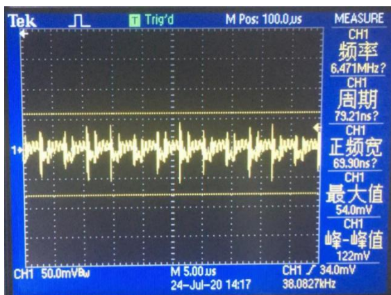
Ripple wave (VIN = 39V IO=2A, 5 ~ 20MHz bandwidth)
