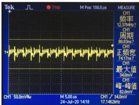
Ripple wave (VIN = 57V, IO = 2A, 5 ~ 20MHz bandwidth)
