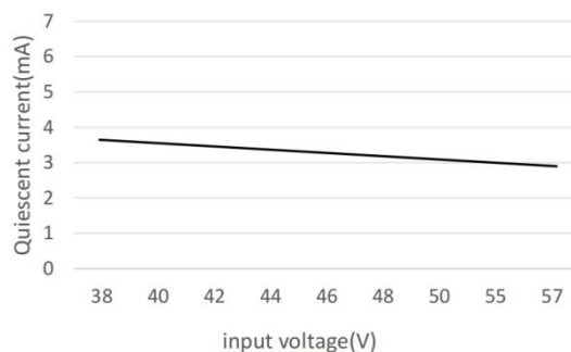
Quiescent current
