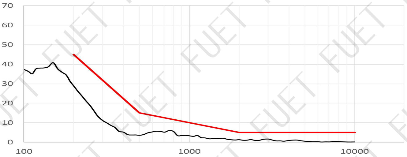
THD/2W/10cm/5CC带障板
