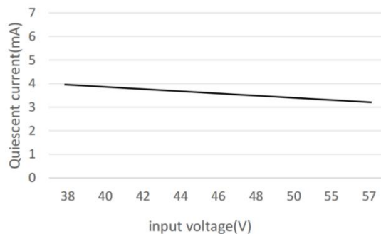
Quiescent current
