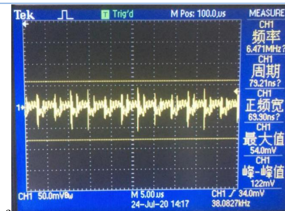
Output ripple (12V/1.1)
