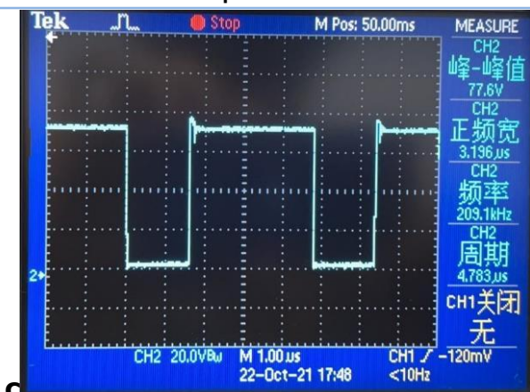
SW switch waveform
