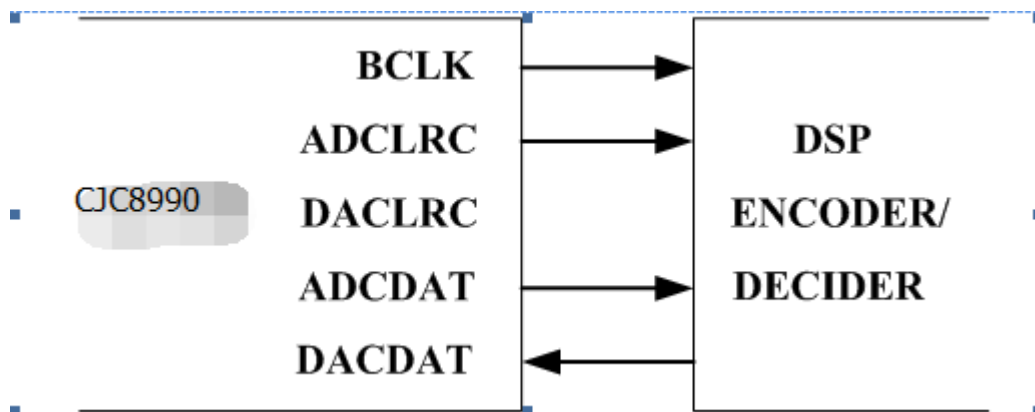
Figure 10 Master Mode
