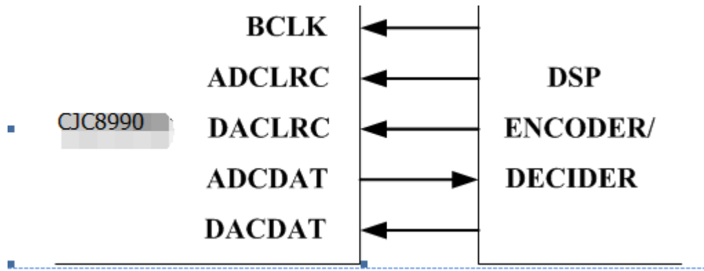
Figure 11 Slave Mode
