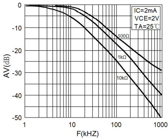
Fig.11 Frequency Response
