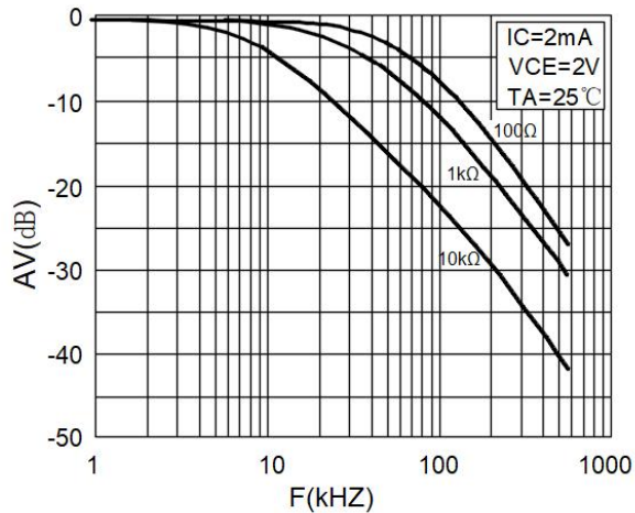
Fig.11 Frequency Response
