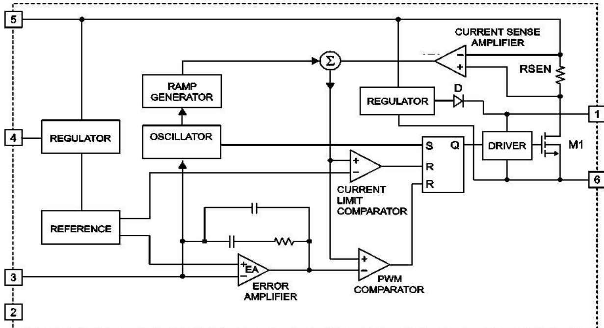
Figure1 Function Block Diagram of TD1466A
