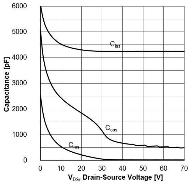
Figure 12. Capacitance Characteristics
