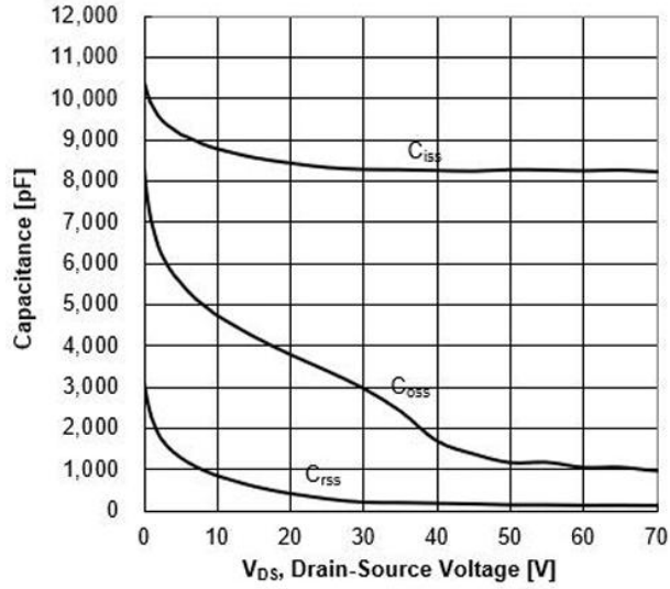
Figure 12. Capacitance Characteristics
