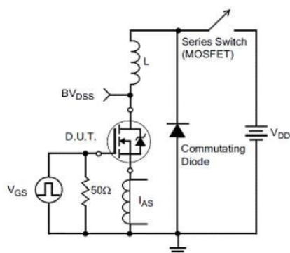
Figure 20. Unclamped Inductive Switching Test Circuit
