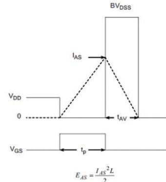
Figure 21. Unclamped Inductive Switching Waveform
