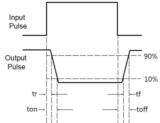
Fig.14 Waveforms of Turn On Time
