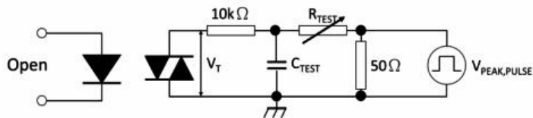
Fig.15 Test Circuits of dv/dt
