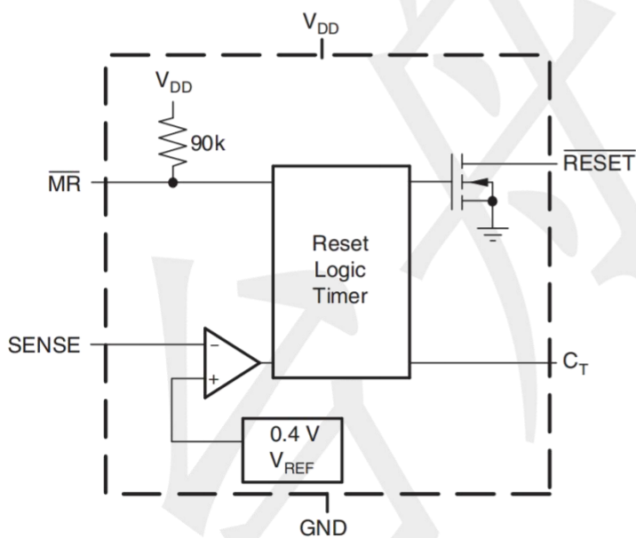
Adjustable-Voltage Version
