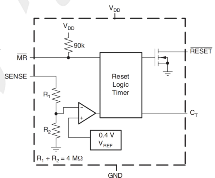
Fixed-Voltage Version
