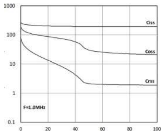
Figure 5: Capacitance Characteristics
