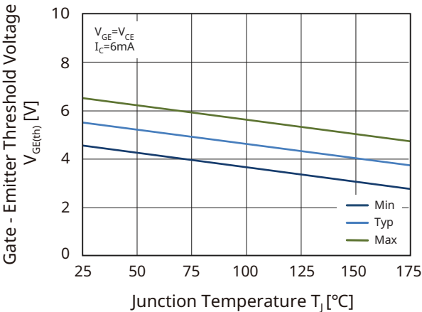
Fig6. Typical Gate-Emmitter Threshold Voltage as a Function of Junction Temperature
