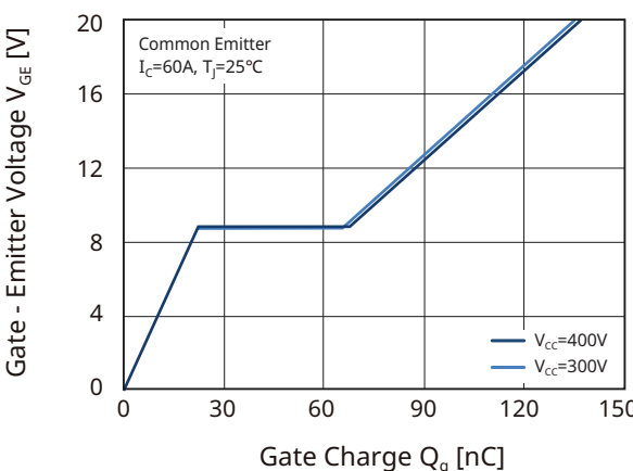
Fig10. Typical Gate Charge
