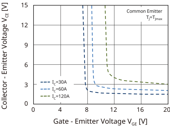
Fig8. Typical Collector-Emmitter Saturation Voltage as a Function of Gate-Emmitter Voltage
