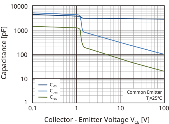
Fig9. Typical Capacitance as a Function of Collector-Emmitter Voltage
