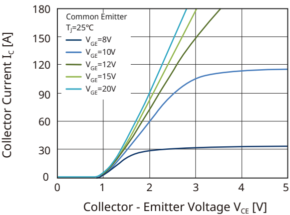
Fig2. Typical Output Characteristic ( I_C vs V_{CE} )@ T_J=25^\circ\text{C}
