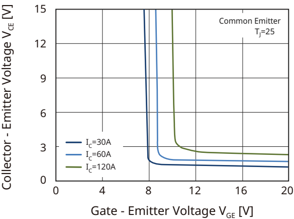
Fig7. Typical Collector-Emmitter Saturation Voltage as a Function of Gate-Emmitter Voltage
