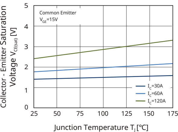
Fig5. Typical Collector-Emmitter Saturation Voltage as a Function of Junction Temperature
