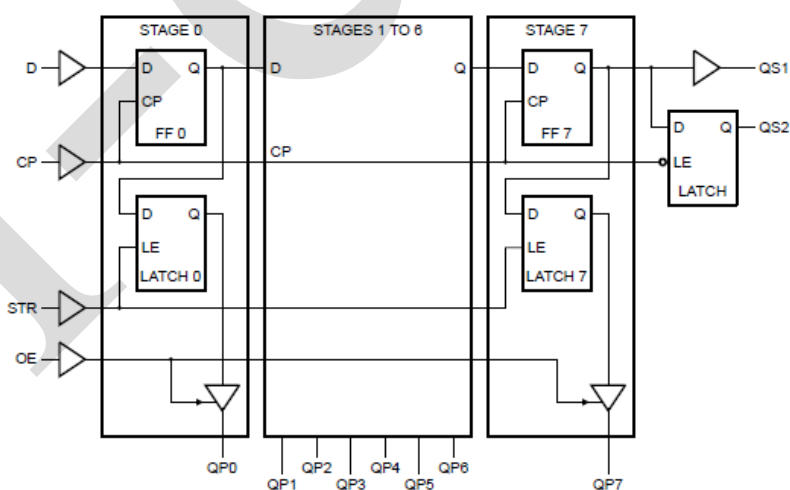
Figure 3. Logic diagram
