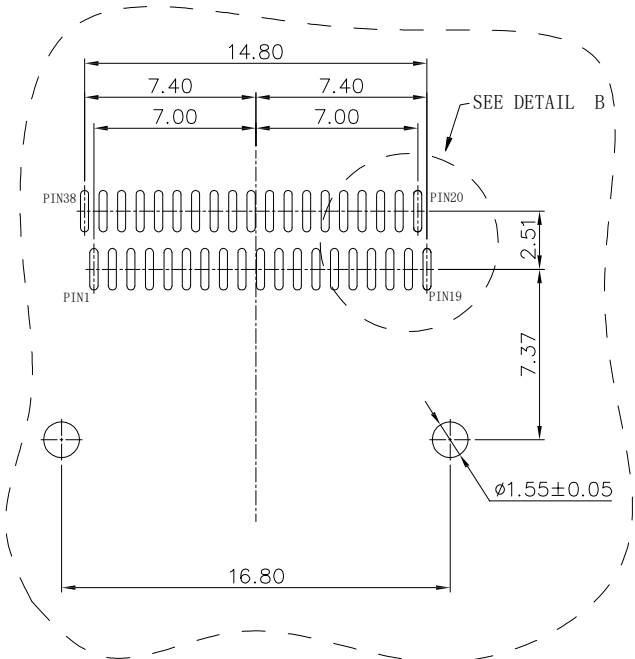
PCB LAYOUT PCB TOLERANCE ±0.05
