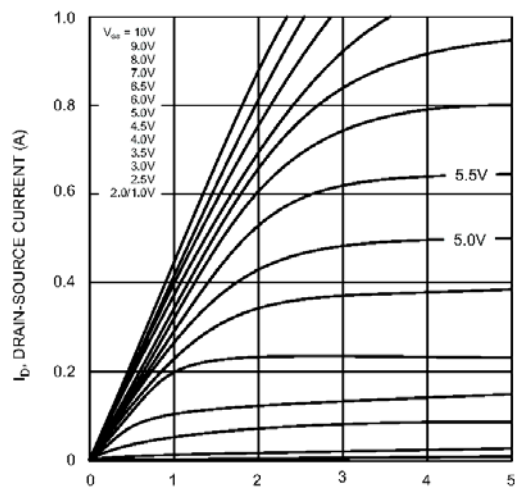
Fig. 1 On-Region Characteristics
