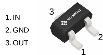
SOT-523 (SOT-523-3)
