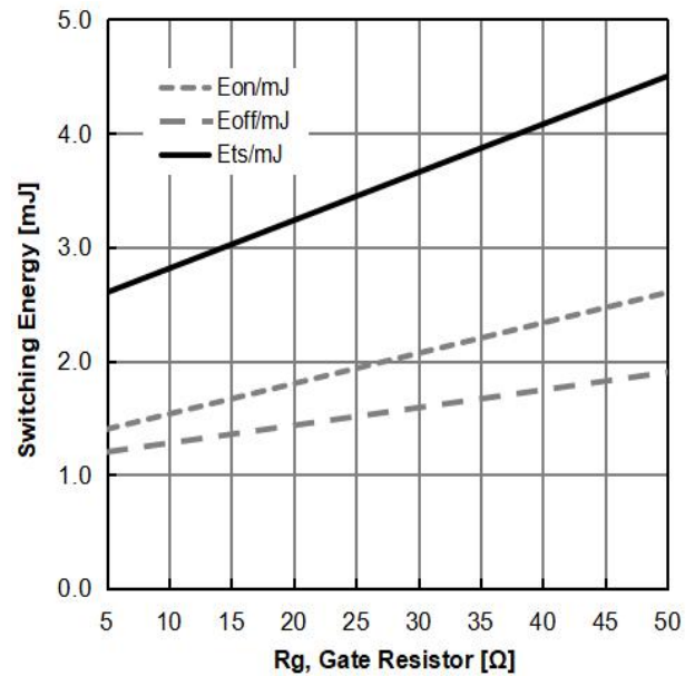
Figure 10: Typical Switching Energy vs. Gate Resistor ( T_J=25^\circ\text{C} , V_{CE}=400\text{V} , V_{GE}=15\text{V} , I_C=60\text{A} )
