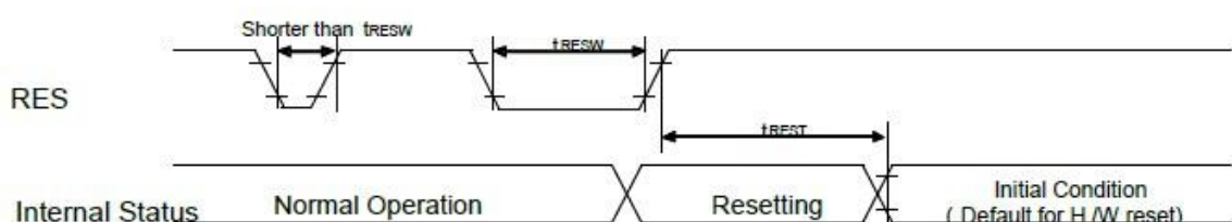
Figure: Reset timing
