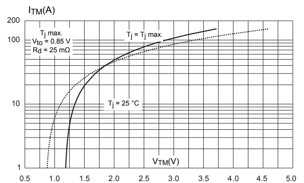
On-state characteristics (maximum values)
