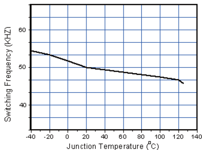
Figure 2. Switching Frequency vs. Temperature
