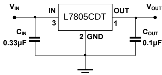
Conventional Circuit
