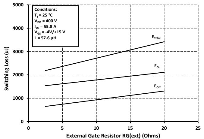
Figure 24. Clamped Inductive Switching Energy vs. R_{gl(ext)}
