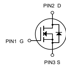
DFN3X3-8L
