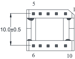
SUGGESTED PADS LAYOUT
