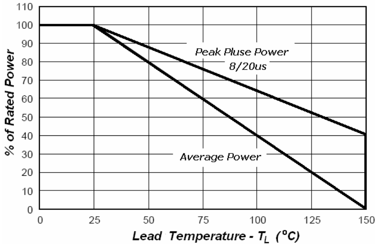
Fig3.Power Derating
