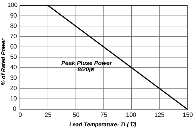
Fig2.Power Derating
