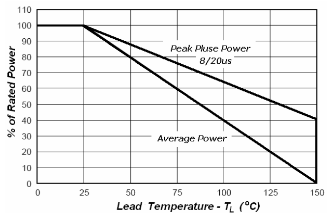
Fig 2. Power Derating
