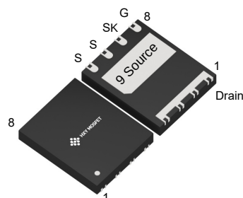
DFN5X6E-8L
