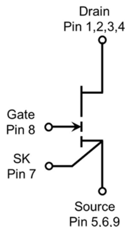
DFN5X6E-8L
