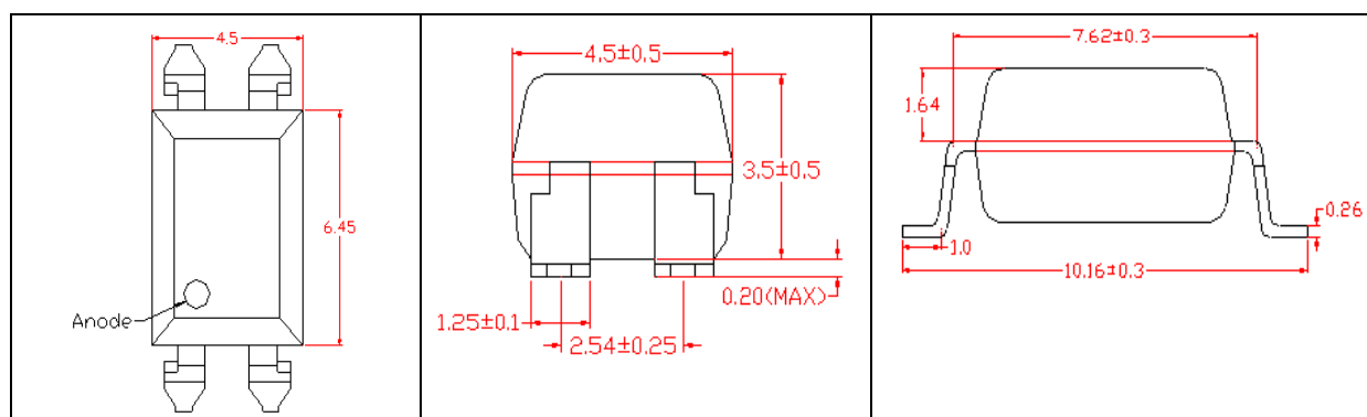
4-pin SMD(SMD-4P)
