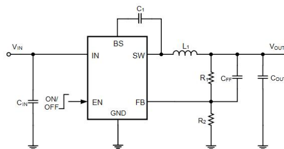
Basic Application Circuit
