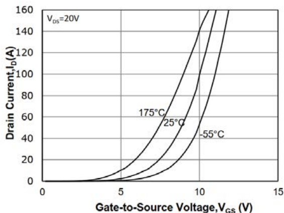
Fig 6: Transfer Characteristic
