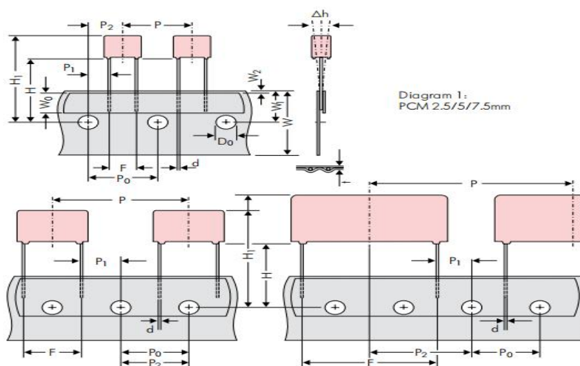
Diagram 2: PCM 10/15 mm
