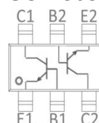
Pin 1
