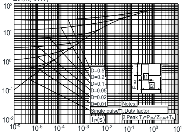
Figure.11: Maximum Effective Transient Thermal Impedance, Junction-to-Ambient Z_{thJA} (^{\circ}\text{C}/\text{W})
