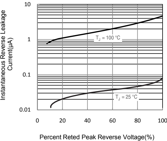
Fig.4 Typicl Reverse Leakage Characteristics
