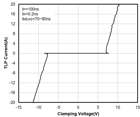
Transmission Line Pulsing (TLP) Voltage (V)
