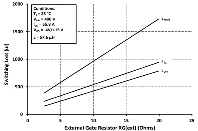
Figure 24. Clamped Inductive Switching Energy vs. R_{(ext)}
