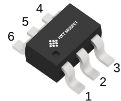
SOT-23-6L (TSOP-6-1.5mm)
