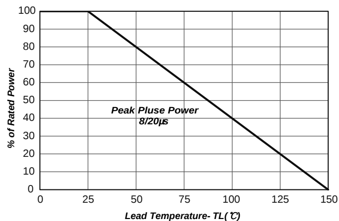
Fig2.Power Derating
