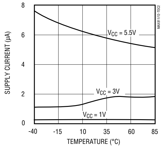
Supply Current vs Temperature (No Load, MAX811L/M/I)
