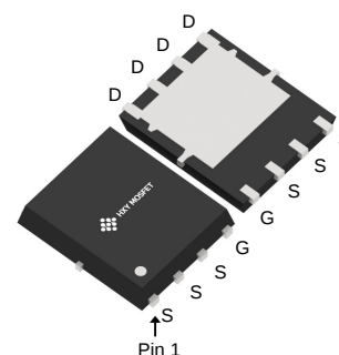
DFN5X6-8L (PowerFLAT-8(5x6))
