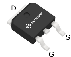
TO-252-2L (TO-252-2(DPAK))
