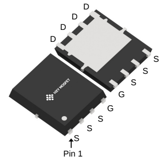
DFN5X6-8L (Power(5x6))
