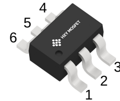
SOT-363 (SOT-363-6)
